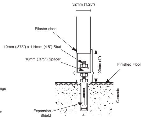
section detail C-C
