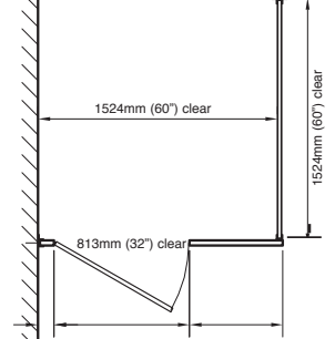
barrier-free plan
