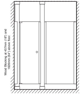
alcove elevation
