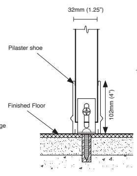
section details C-C
