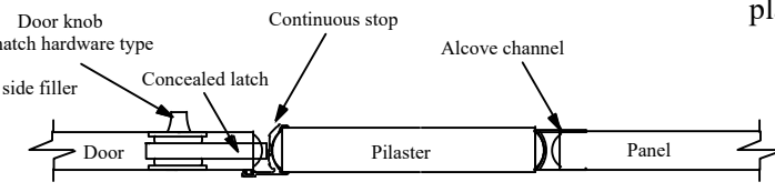
plan detail E-E
