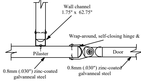
plan detail A-A
