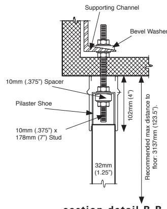
section detail B-B
