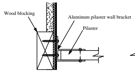
plan detail D-D
