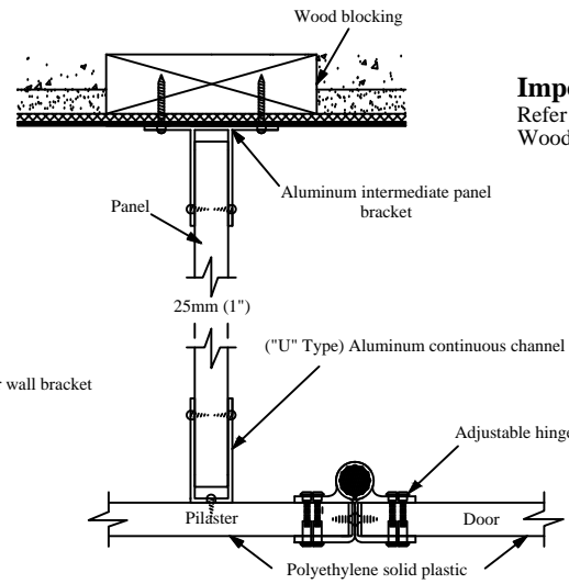
plan detail A-A
